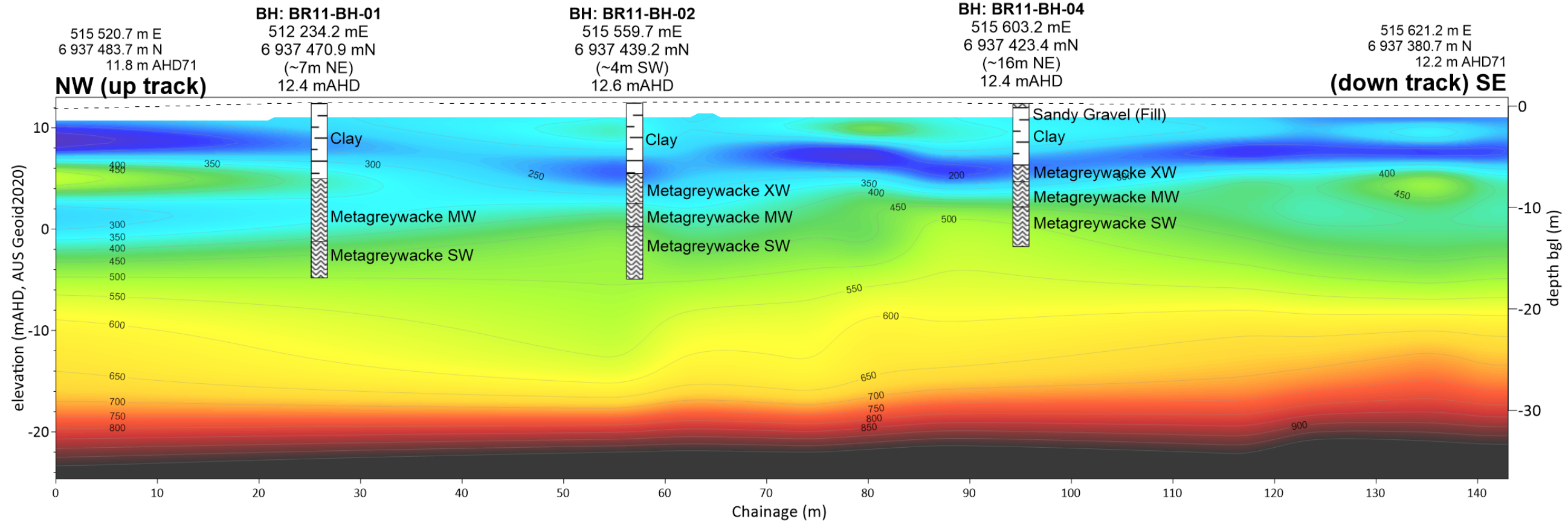
Seismic Line MASW AU-GP 164-3
